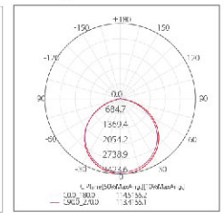
100W glass
